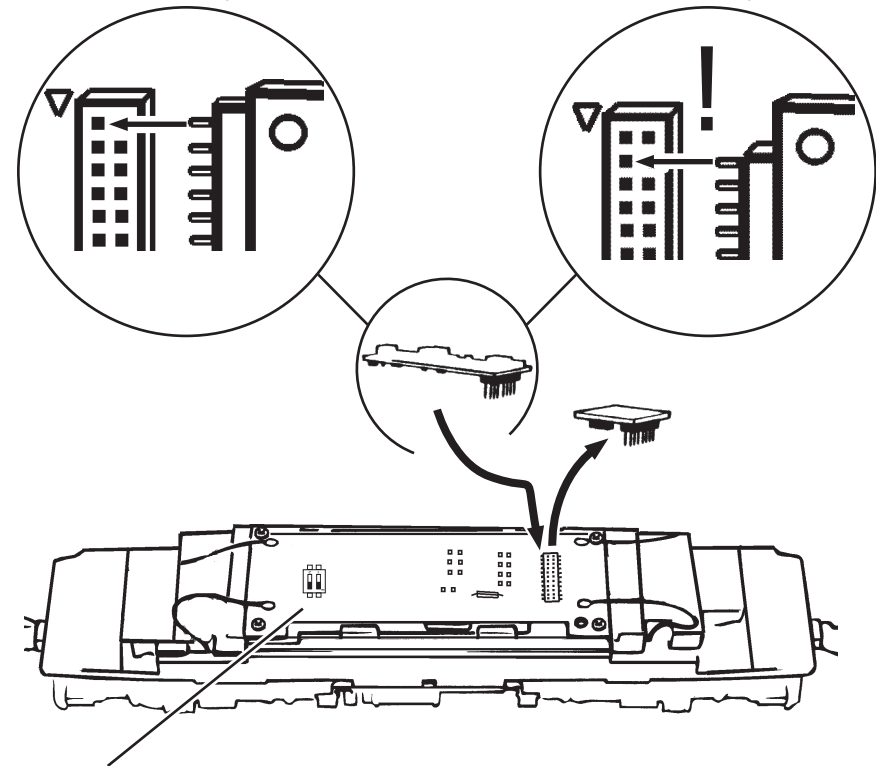
Decoder 22-pin
